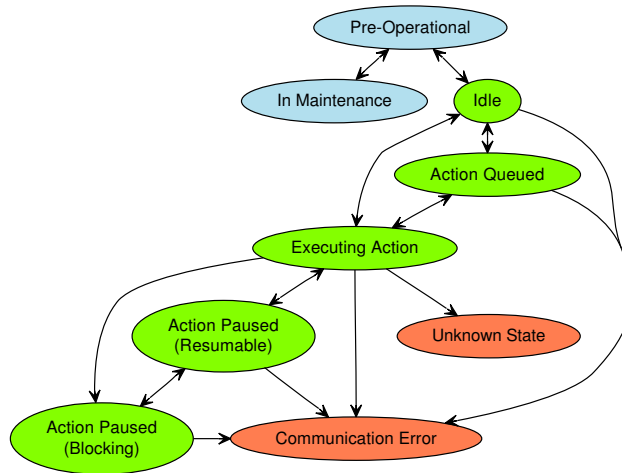
Fig. 5. State-machine of SEE modes and possible transitions. Blue modes denote long-term unavailability. The green modes are for runtime of the SEE and require active communication. Otherwise, the MES internally assumes the Communication Error mode. If the execution of an action aborts, the SEE may not know the exact state of its configuration and the contained products. In that case, it will switch to the Unknown State error mode that can only be resolved by human intervention.
