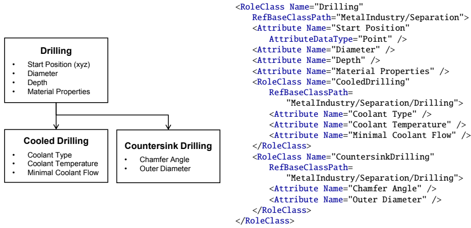
Fig. 3. Excerpt of the process hierarchy and its representation in AutomationML. The arrows indicate the inheritance of attributes from the parent processes. All attributes may refer to custom (structured) datatypes.
